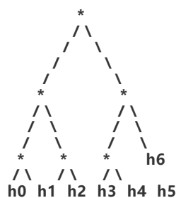
A SimpleTree with 7 elements
